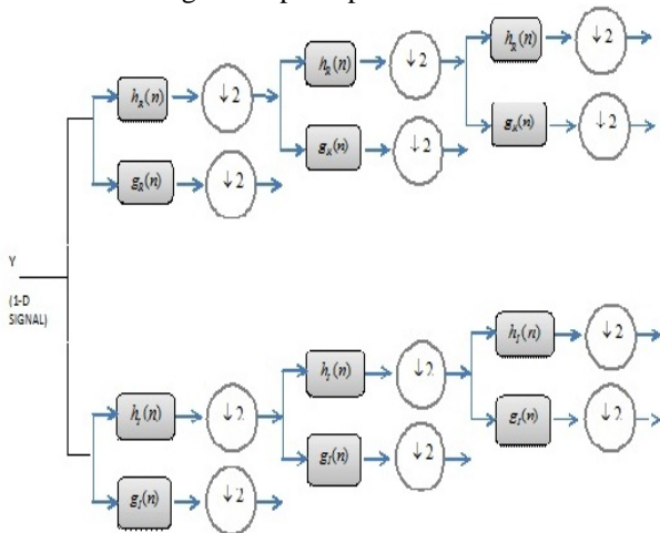
Fig. 2 Analysis of Dual Tree Complex Wavelet Transform
